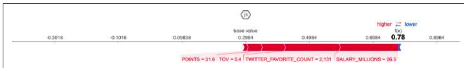
Figure 5-43. SHAP output xgboost
