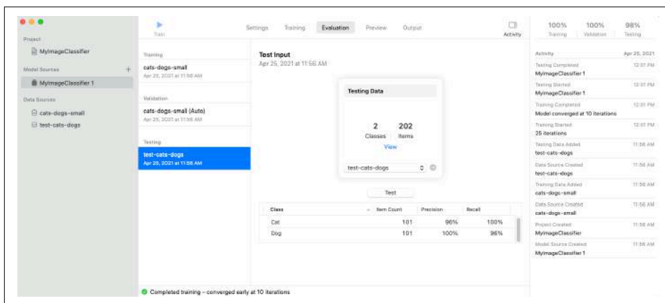
Figure 5-17. Trained model
