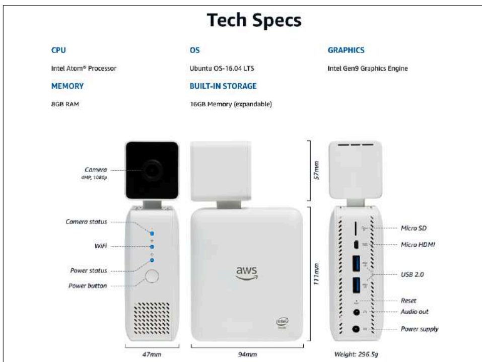
Figure 7-14. DeepLens
