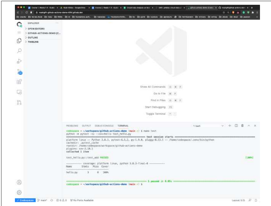
Figure 1-5. GitHub Codespaces
