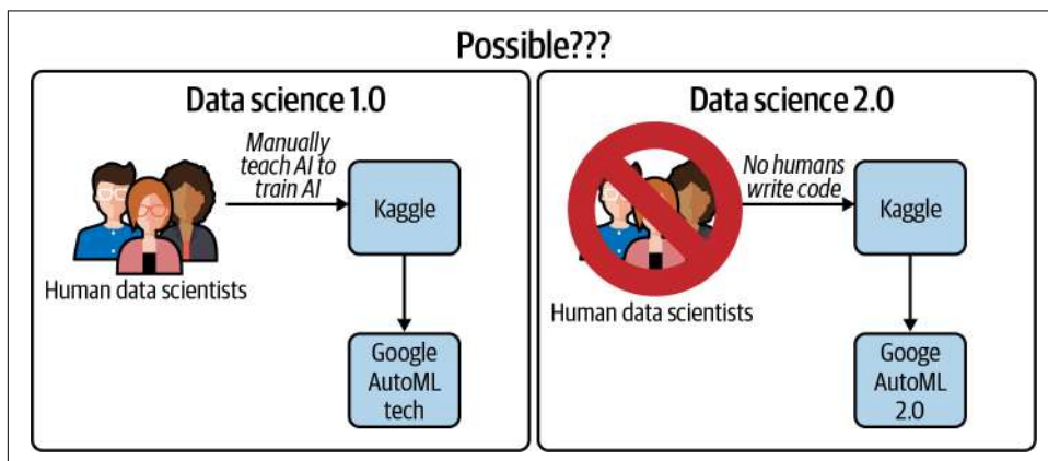
Figure 5-4. Kaggle automation
