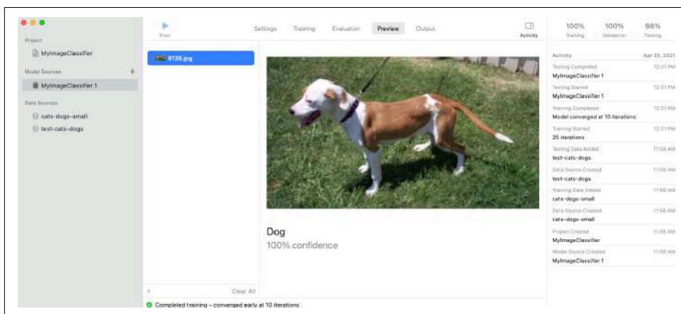
Figure 5-18. Preview
