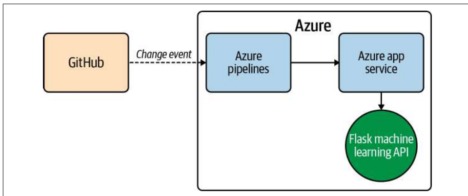
Figure 2-20. MLOps overview
