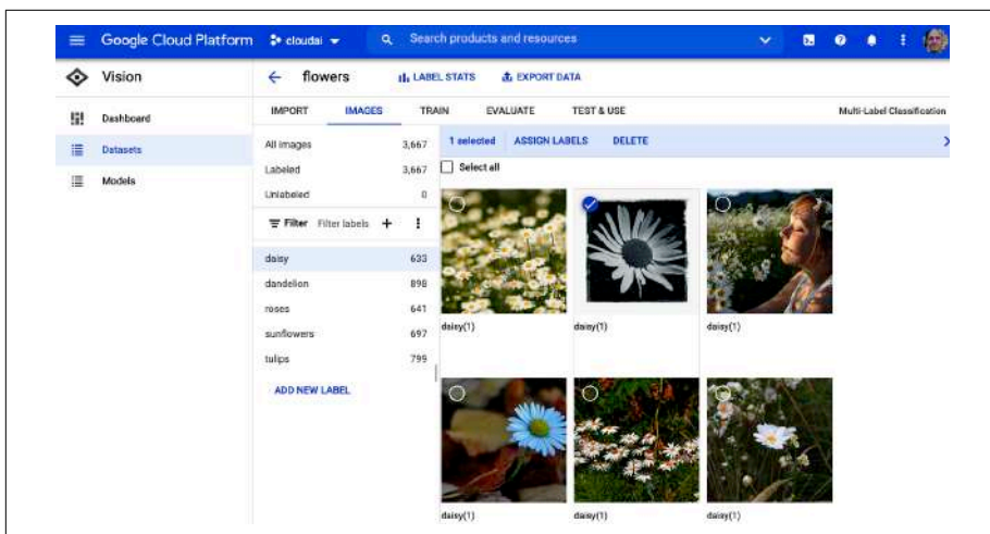
Figure 5-23. Inspect data
